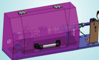
Keylock Set durability testing
