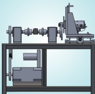
Motor Test Bench Setup
